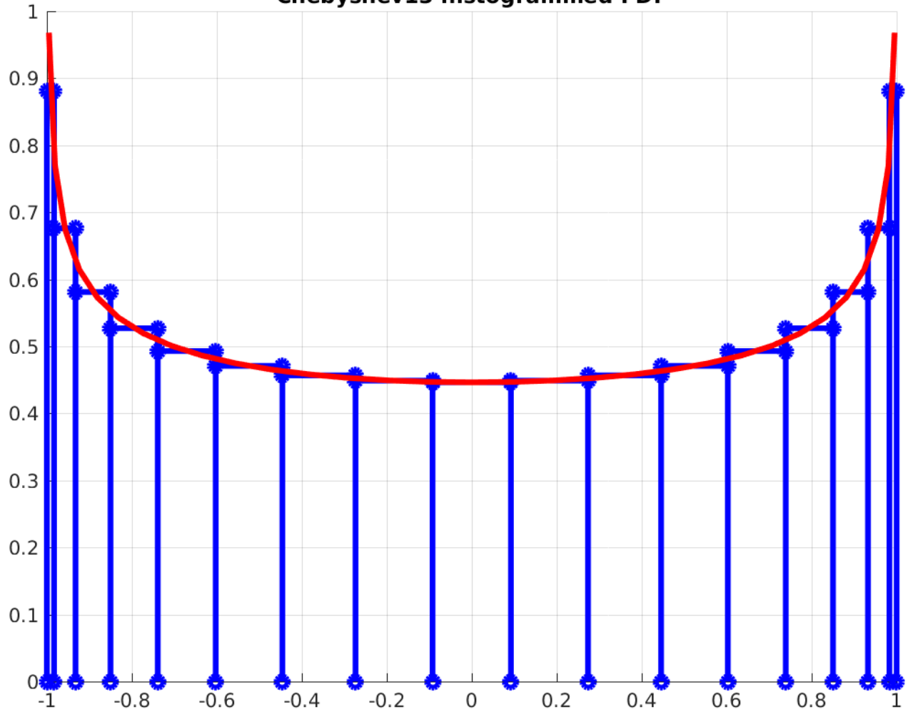
Chebyshev13 histogrammed PDF
