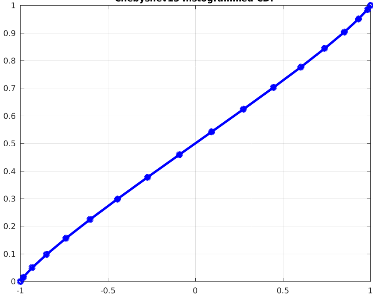
Chebyshev13 histogrammed CDF
