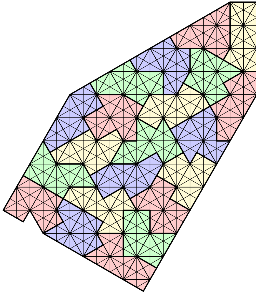
Figure : Boat solution.
