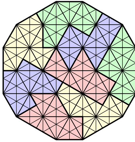
Figure : Serenity solution.
