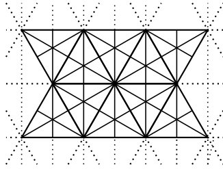
Figure : Triangles subdivided
