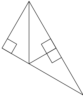
Figure : A tridrafter using three contiguous elements
