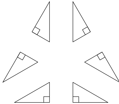
Figure : The six orientation of an element
