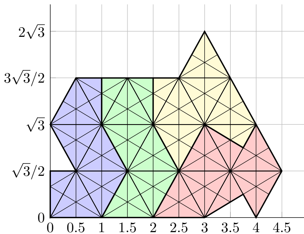
Figure : How 4 tiles cover the Trinity region; (x, y) coordinate system.
