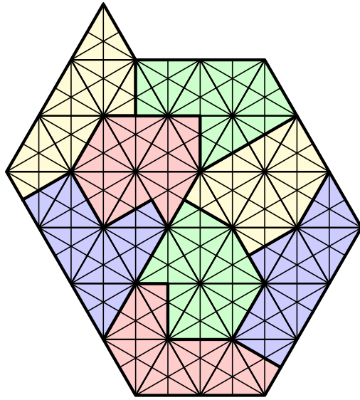
Figure : Whale solution.
