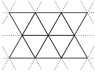
Figure : The isometric grid
