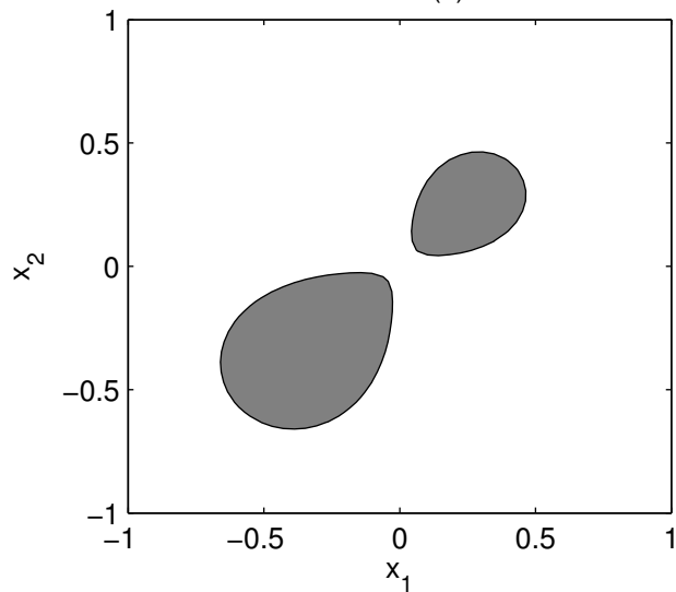
The event u(x) > 0.9
