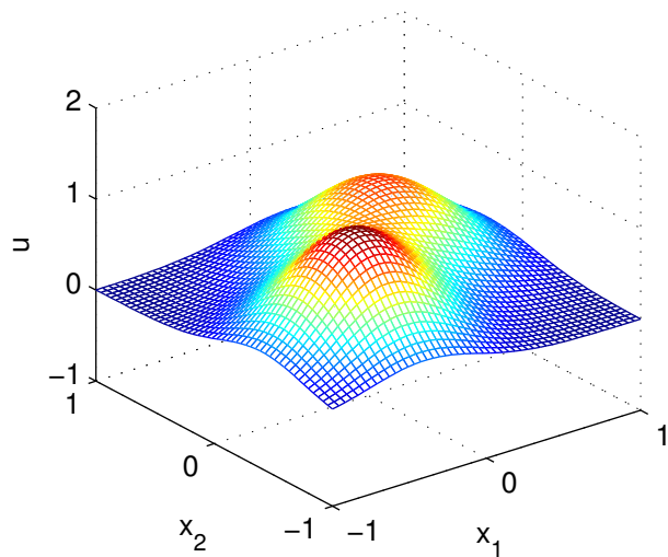
response surface u(x)
