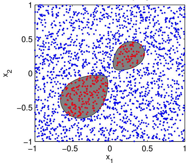
Monte Carlo Sampling
