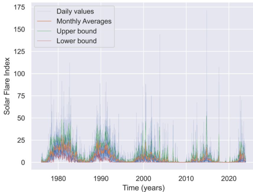
Daily and monthly Solar Flare Indices for the period of 1976–2023. Raw data by Kandili Observatory, processing and plots generated by me (Python, Seaborn and Matplotlib).
