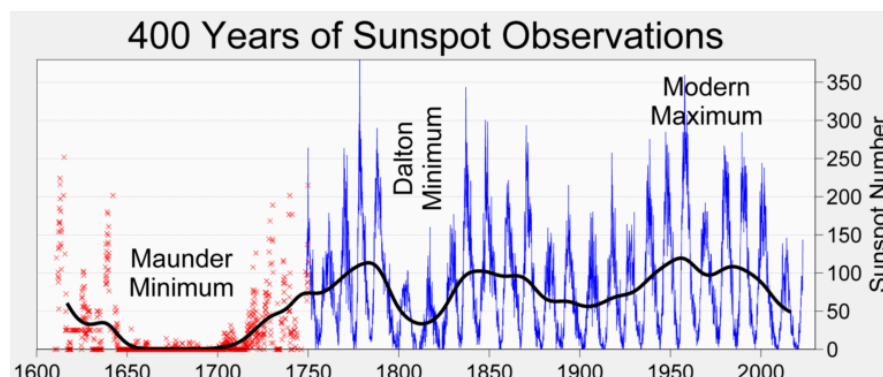
Plot showing historical sunspot records, by Robert A. Rohde (part of the Global Warming Art project). Image in the public domain, under a CC BY-SA 3.0 license ( source ).
