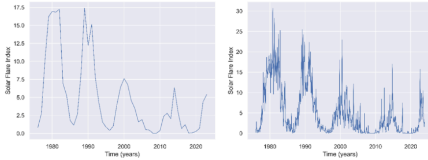
Yearly and monthly Solar Flare Indices for the period of 1976–2023. Raw data by Kandili Observatory, processing and plots generated by me (Python, Seaborn and Matplotlib). Image by Pau Blasco i Roca.
