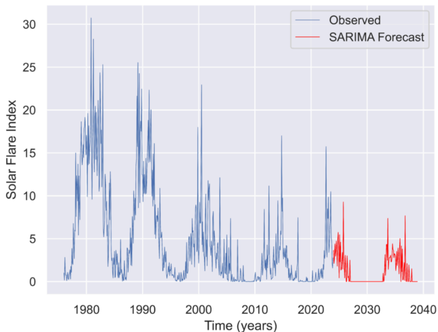
Prediction of the SARIMA model, generated by me (Python, Seaborn, Matplotlib, Numpy and Statsmodels). Image by Pau Blasco i Roca.
