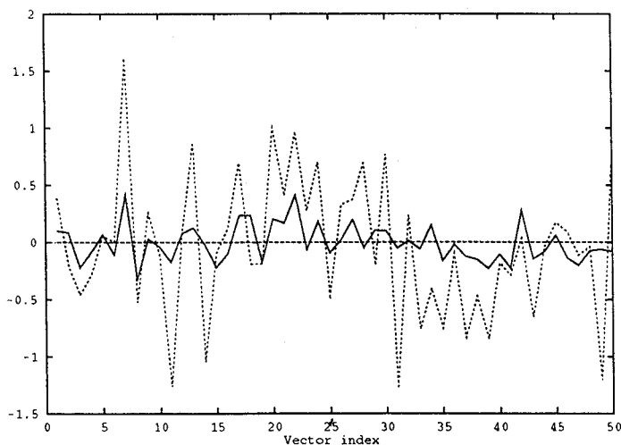
Figure 2. The first 50 components of the difference between the Hessian vector products obtained by using the second order adjoint and the finite-difference techniques scaled by a factor 1.E09 after 15 iterations using the adjoint truncated-Newton algorithm where the differencing parameter is chosen as h_1 = h (solid line), h_2 = h \times 1.E-01 (dotted line) and h_3 = h \times 1.E+03 (dashed line, which coincides with the x -axis) instead of h in the original truncated-Newton algorithm, respectively.
