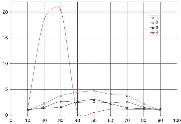
Figure 9. Relative importance of sensors from the viewpoint of different criteria. 1— \|\delta T_{int}^{obs}\| , 2— \|\delta \nabla \varepsilon\| , 3— \|\delta T_0\| , 4— |(\psi, \delta \nabla \varepsilon)| .
