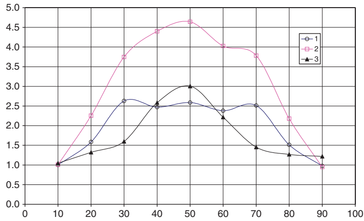
Figure 8. Relative importance of sensors from the viewpoint of different criteria. 1— \|\delta T_{int}^{obs}\| , 2— \|\delta \nabla \varepsilon\| , 3— \|\delta T_0\| .
