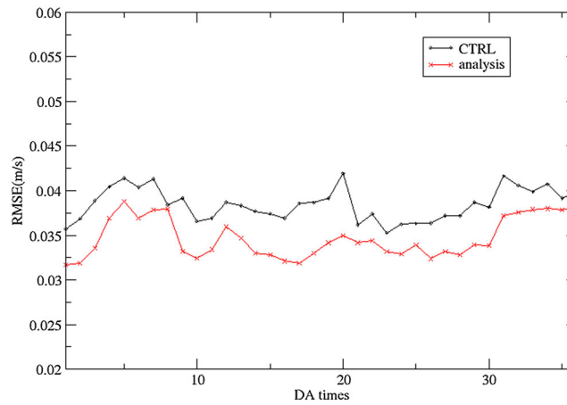
Figure 11. Error in the x -direction component of velocity (unit: m/s), before (marked as 'CTRL') and after (marked as 'analysis') ensemble Kalman filter data assimilation. RMSE, root mean square error.
