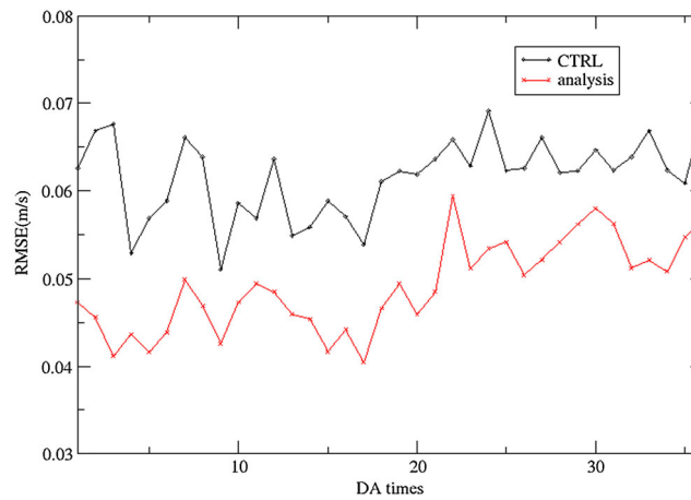
Figure 5. Error in the x-direction component of velocity (unit: m/s), before (marked as ‘CTRL’) and after (marked as ‘analysis’) ensemble Kalman filter (EnKF) data assimilation.
