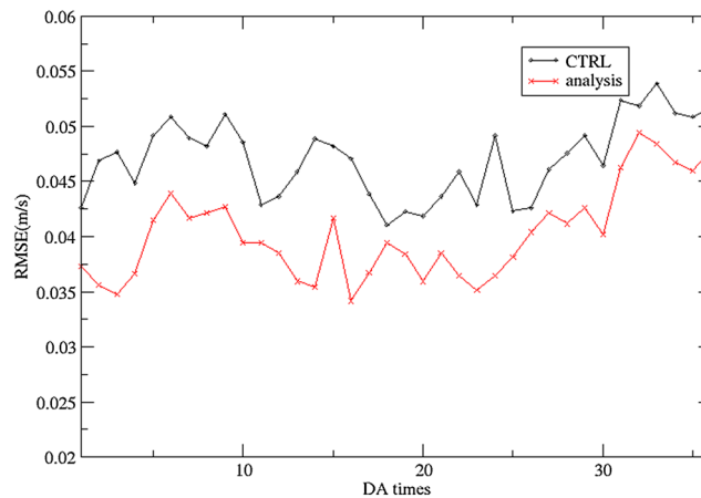
Figure 9. Error in the x-direction component of velocity (unit: m/s), before (marked as ‘CTRL’) and after (marked as ‘analysis’) ensemble Kalman filter method data assimilation.
