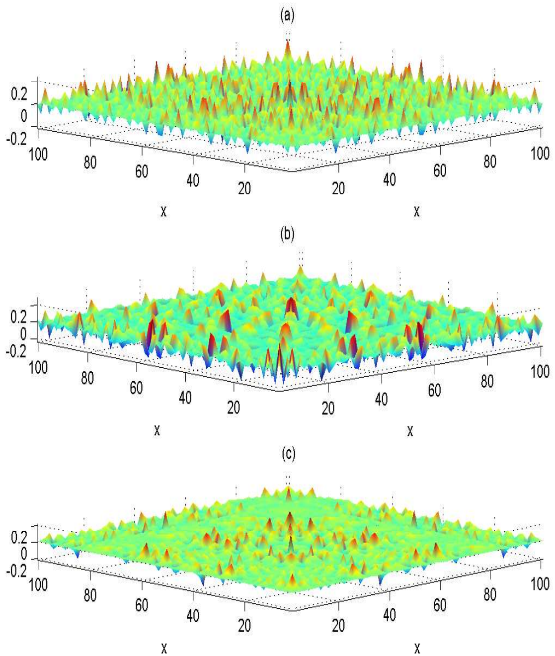
Figure 6. Analysis error covariance using 200 particles. (a) after t = 20 time units , (b) after t = 100 time units and (c) after t = 250 time units, linear observation operator case
