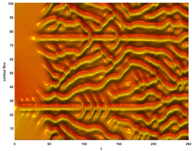
Figure 1. Contours for the time evolution for the K-S equation
