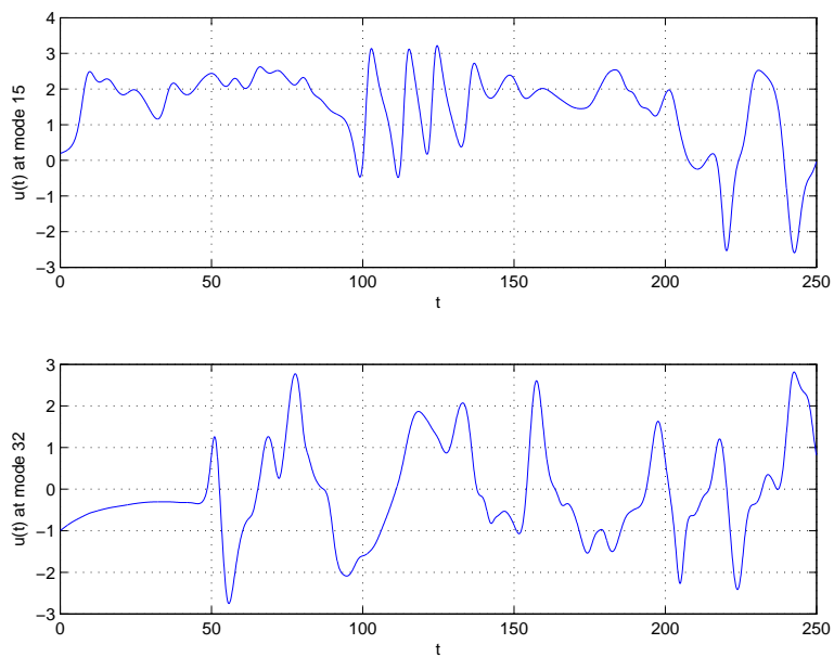
Figure 2. K-S solution at different spatial positions
