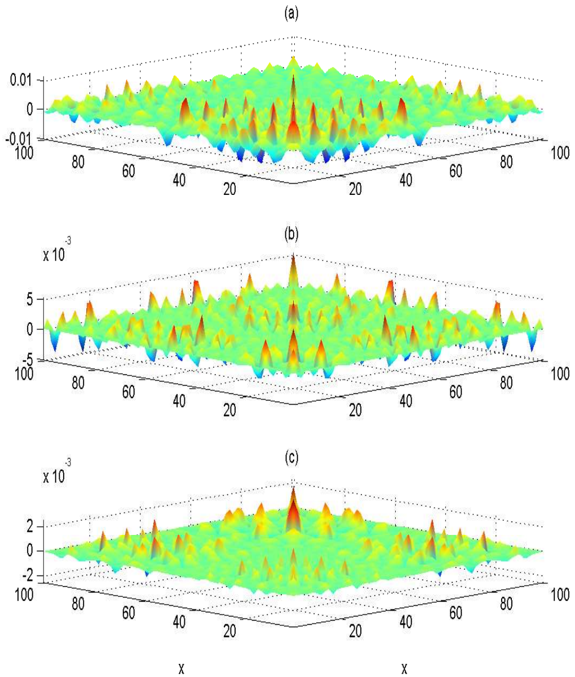
Figure 10. Analysis error covariance using 100 ensemble members. (a) after t = 20 time units , (b) after t = 100 time units and (c) after t = 250 time units, linear observation operator case
