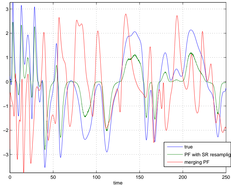
Figure 8. PF with the SR resampling and MPF solutions for the K-S equation model, linear observation operator case
