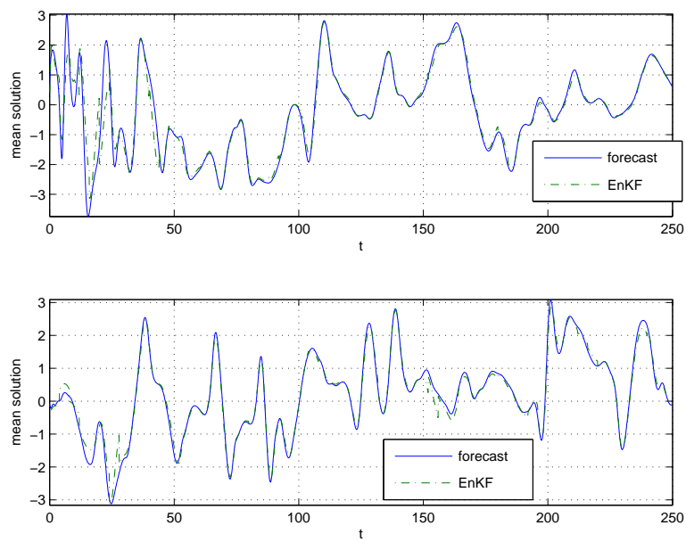
Figure 9. Forecast and EnKF filter mean K-S solution at two different locations, linear observation operator case
