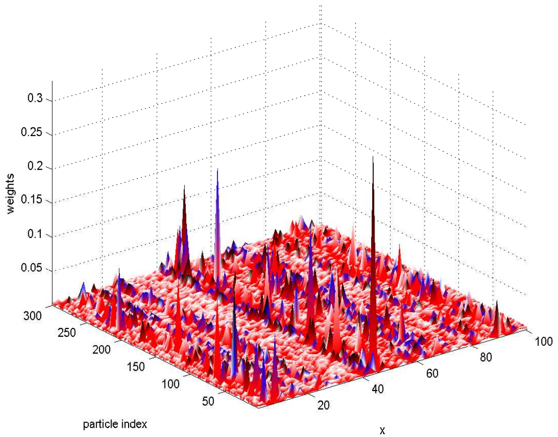
Figure 4. Weights distribution at a fixed time. 300 particles at the final time t = 250 , using the systematic resampling method, linear observation operator case
