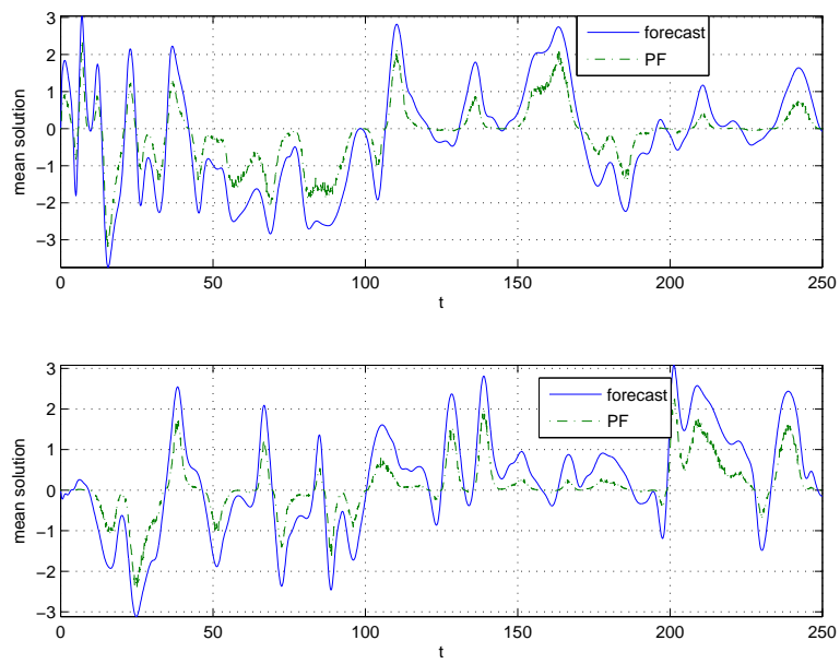
Figure 5. Forecast and PF filter mean K-S solution at two different locations, linear observation operator case
