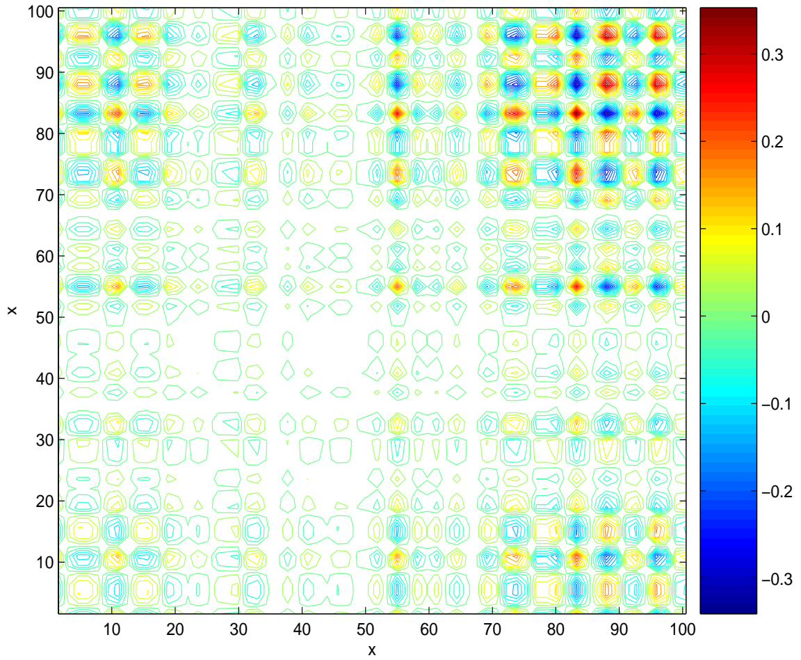
Figure 13. Contours of the analysis error covariance after 250 time units using 100 ensemble members, linear observation operator case
