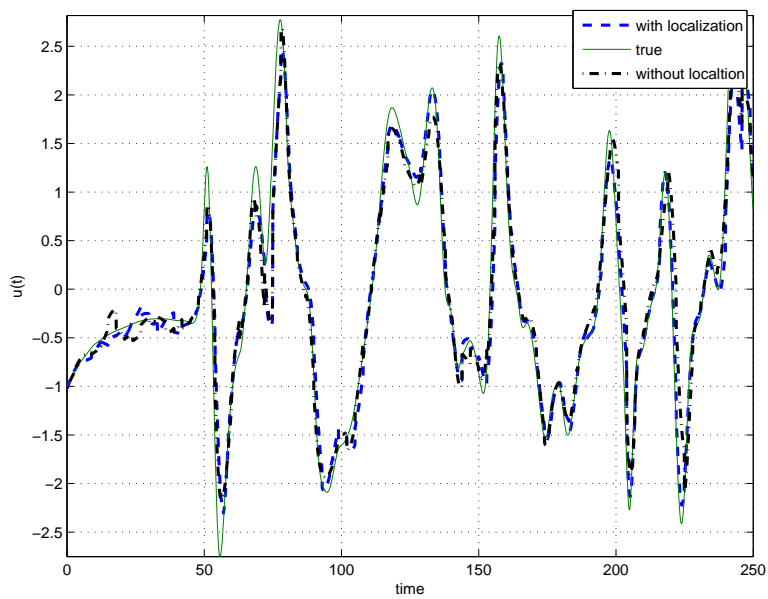
Figure 12. EnKF solutions with and without the inflation and localization covariance feature, linear observation operator case
