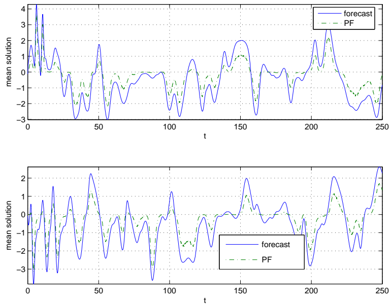
Figure 16. Means of the K-S solution using SIR particle filter, nonlinear observation operator case
