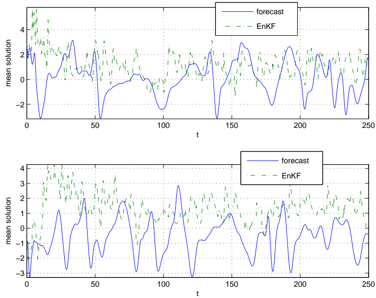
Figure 15. Means of the forecast and the EnKF filtered K-S solution in the case of a nonlinear observation operator \mathcal{H}u = u^2 , nonlinear observation operator case
