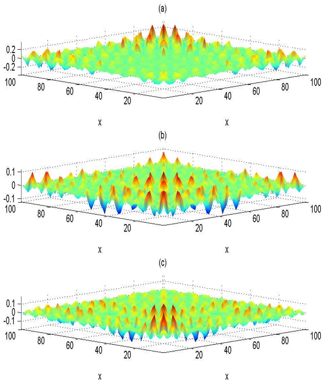
Figure 14. Analysis error covariance using 100 ensemble members. (a) after t = 20 time units, (b) after t = 100 time units and (c) after t = 250 time units, linear observation operator case
