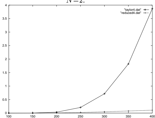
Figure 3: The relative error with increasing R . The approximation order varies from N=0 to 5. Taylor method is solid, reduced basis dashed.
