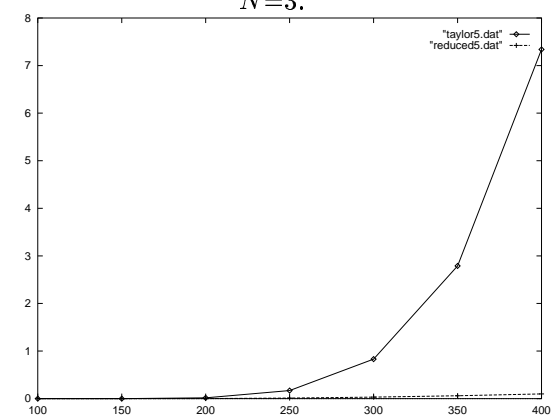
Figure 3: The relative error with increasing R . The approximation order varies from N=0 to 5. Taylor method is solid, reduced basis dashed.
