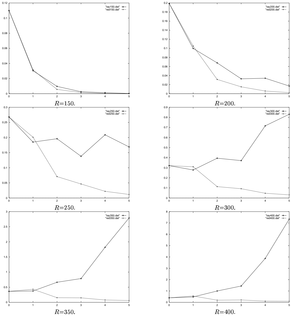
Figure 2: The relative error versus approximation order N . The value of R varies from 150 to 400. Taylor method is solid, reduced basis dashed.
