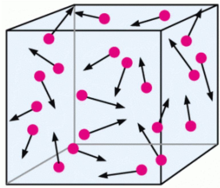
Figure 6.1: Particles with Momentum and Weak Attraction
