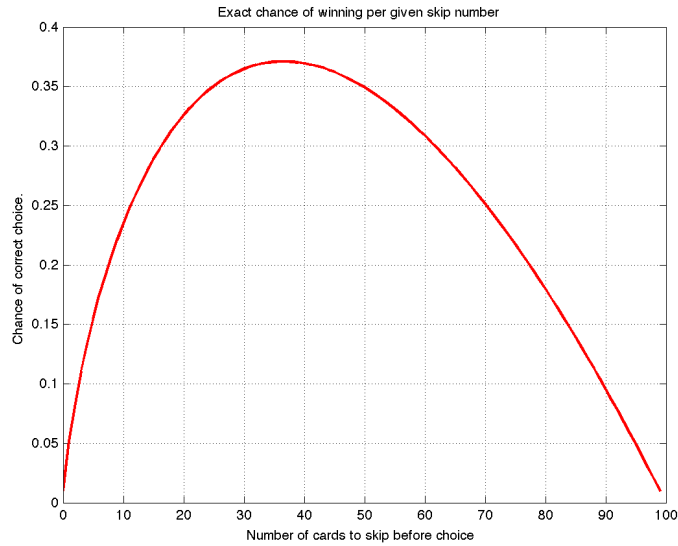
Figure 3.2: The exact probability of winning high card with a deck of 100
