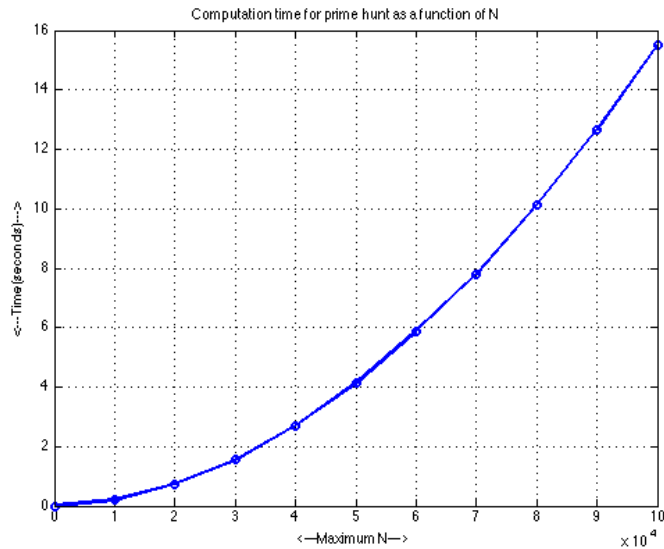
Figure 4.2: Computing primes from 1 to N gets quadratically harder
