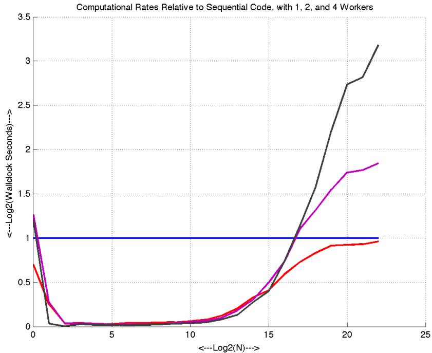
Figure 2.2: Rates for 1, 2, 4 workers, relative to sequential code
