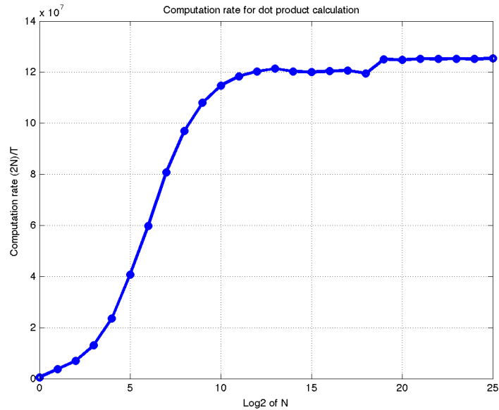
Figure 7.3: Computational Rate for the Dot Product
