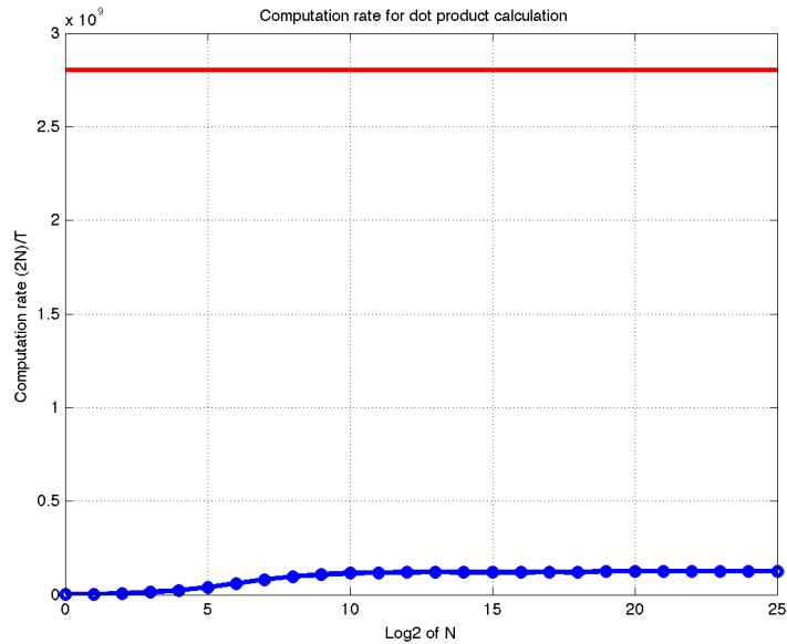
Figure 7.4: Comparison of Dot Product Rate to Maximum
