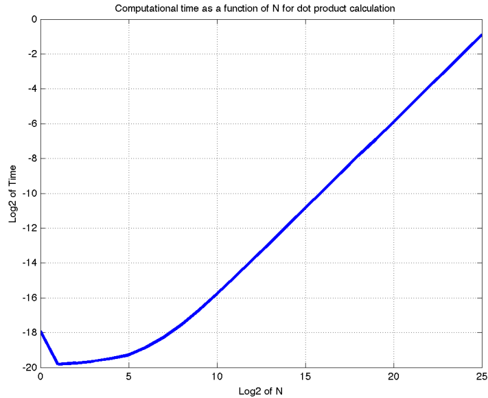
Figure 7.2: Computational Time for the Dot Product
