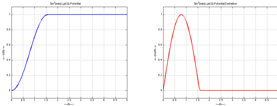
Figure 6.2: The \sin^2 Potential V(d) and Derivative V'(d)
