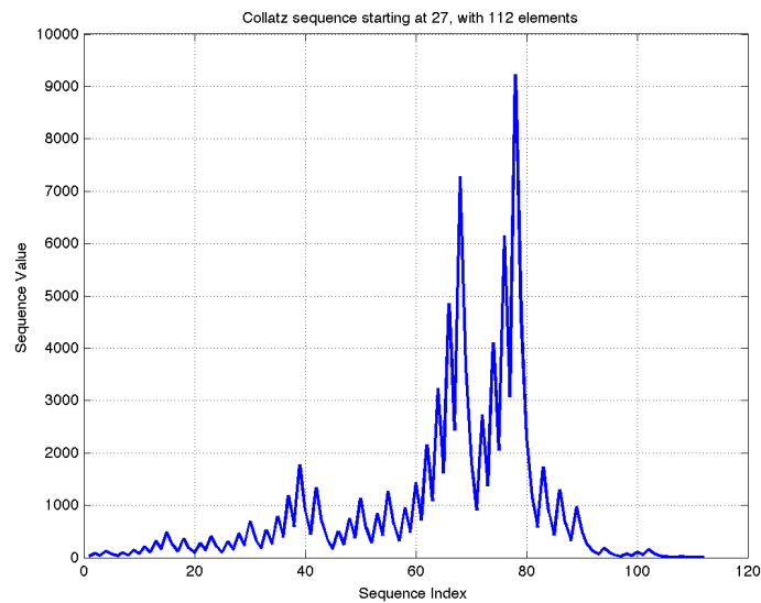
Figure 5.1: Collatz sequence for 27
