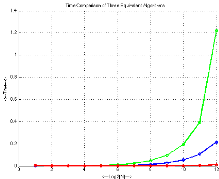
Figure 7.5: Absolute Time Comparison for Three Equivalent Algorithms
