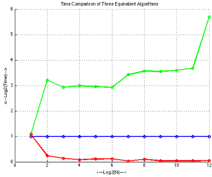
Figure 7.6: Relative Time Comparison for Three Equivalent Algorithms
