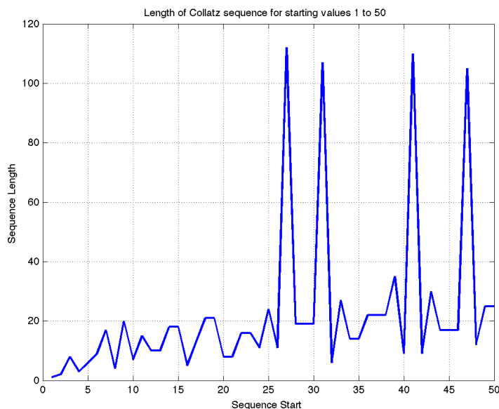
Figure 5.2: Collatz sequence lengths for 1 to 50
