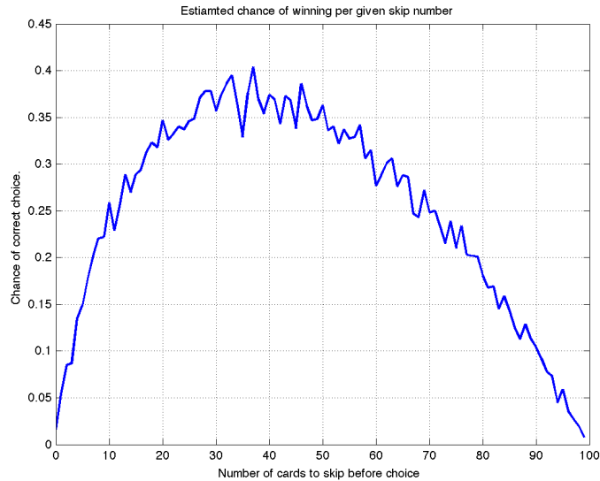
Figure 3.3: The estimated probabilities, with a deck of 100, and 1,000 trials.
