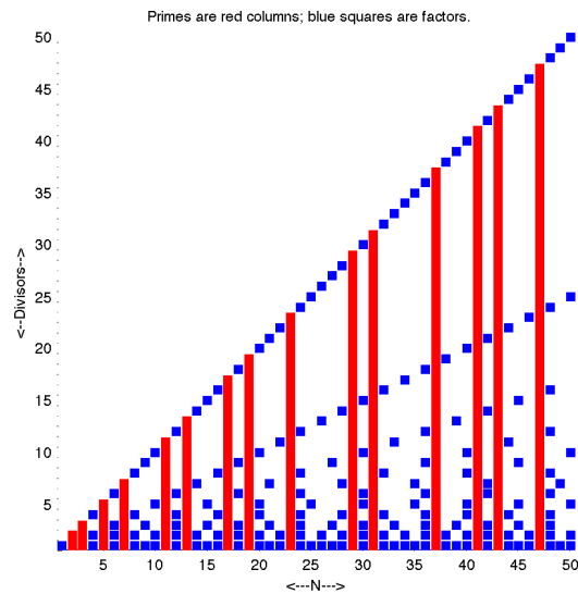
Figure 4.1: Primes (red columns) are scattered among the integers
