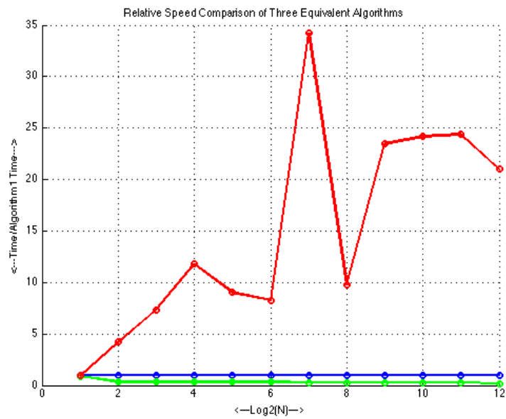
Figure 7.7: Relative Speed Comparison for Three Equivalent Algorithms
