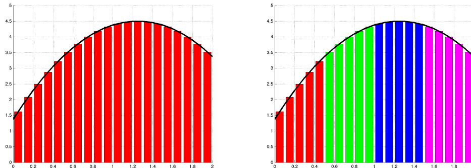
Figure 2.1: Sequential and Parallel Integral Estimates by Quadrature
