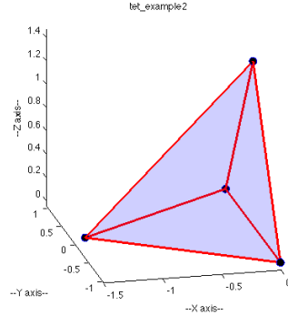
Figure 3: Example Tetrahedron \mathbf{Tet2} = \{ \{-\sqrt{2}, 0, 0\}, \{0, 1, 0\}, \{0, -1, 0\}, \{0, 0, \sqrt{2}\} \}
