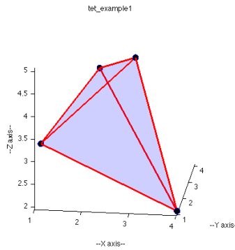
Figure 2: Example Tetrahedron Tet1 = \{\{1,2,3\},\{4,1,2\},\{2,4,4\},\{3,2,5\}\}
