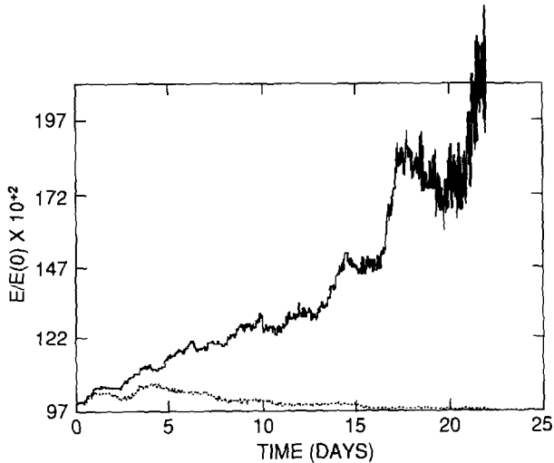
FIG. 3. Potential enstrophy as a function of the time (days) for the non-conserving rectangular finite-element scheme (continuous line), \Delta t_{\text{RECT}} = 900 s, and for the energy conserving scheme (dashed line).
