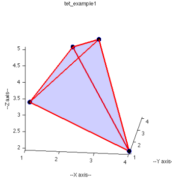
Figure 2: Example Tetrahedron \mathbf{Tet1} = \{\{1,2,3\},\{4,1,2\},\{2,4,4\},\{3,2,5\}\}
