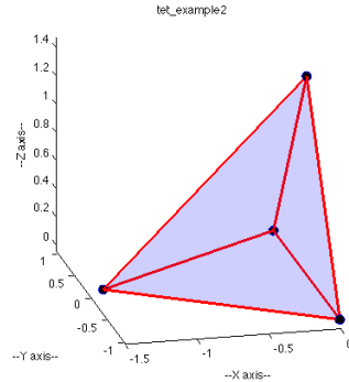
Figure 3: Example Tetrahedron Tet2 = \{ \{-\sqrt{2}, 0, 0\}, \{0, 1, 0\}, \{0, -1, 0\}, \{0, 0, \sqrt{2}\} \}
