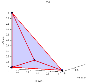
Figure 1: The Reference Tetrahedron \mathbf{Tref} = \{\{1,0,0\},\{0,1,0\},\{0,0,1\},\{0,0,0\}\}
